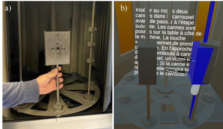
Fig. 4. Installation of a substrate holder rod: a) view of the real system; b) view in the “Virtual PVD” application.
