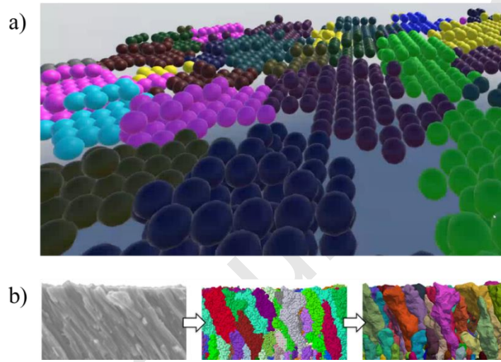
Fig. 10. Film growth: a) atomic view; b) columnar view [20].
