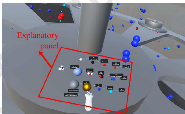
Fig. 6. Gas molecules and atoms in the atmosphere and explanatory panel.
