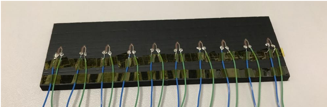
Figure 8: Printed temperature sensors (Cu/CuNi-thermocouples) on CFRP test samples
