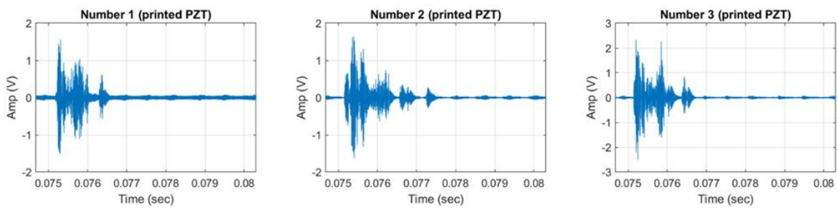
Figure 5: PZT sensor signals / impact detection on CFRP test samples
