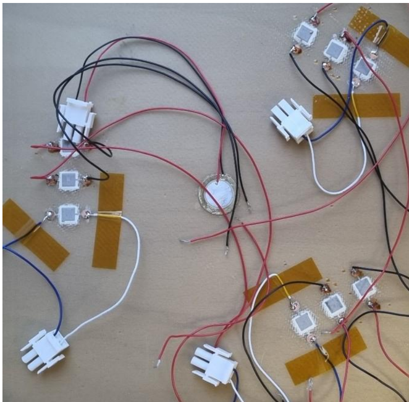
Figure 6: Piezoelectric sensors on GFK sample
