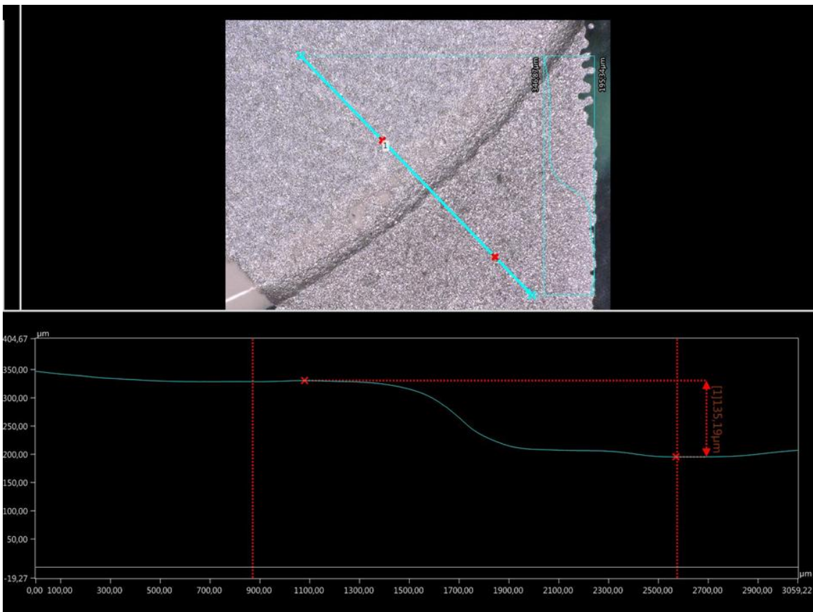
Figure 3: Investigation of layer thickness of piezoelectric layer using a Keyence VHX digital microscope
