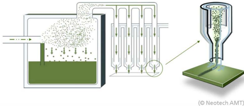
Figure 7: Aerosol Jet ® printing process
