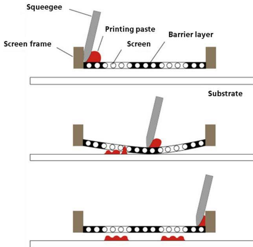
Figure 1: Schematic diagram of the screen-printing process
