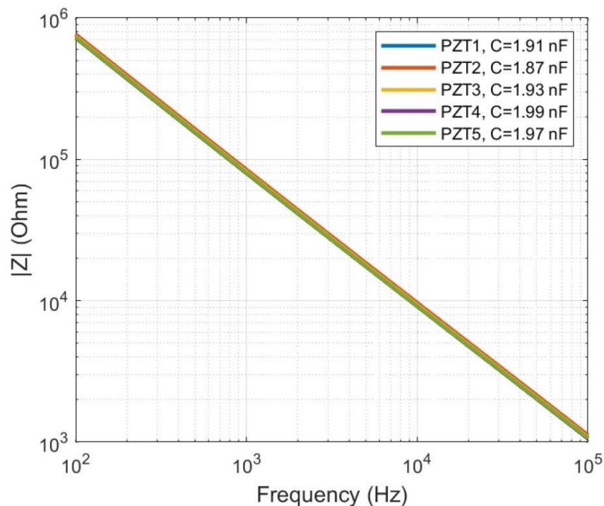
Figure 4: Variation of the modulus of the impedances with frequency measured for 5 similar printed piezoelectric elements. A good repeatability of printed piezoelectric sensors process can be observed.
