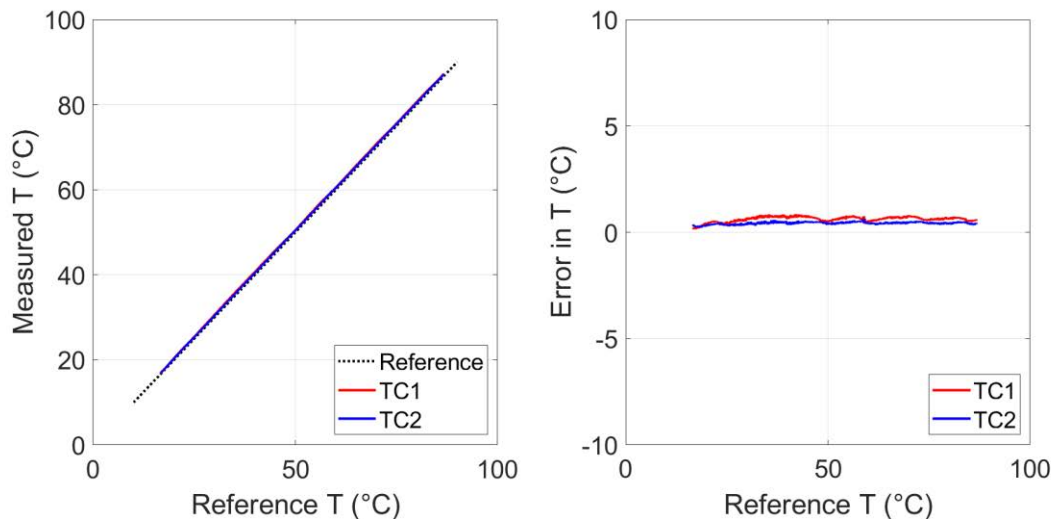
Figure 9: Printed temperature sensors (Cu/CuNi-thermocouples) temperature measurements in comparison with a reference type K thermocouple.
