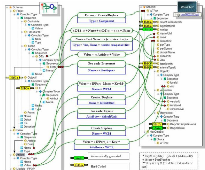
Figure 16 : Correspondence description between IPOP and WindChill structures.
