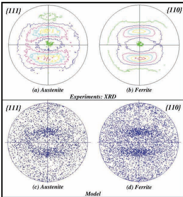
Fig. 5. (a)–(b) Recorded: FCC {111} and BCC {110} pole figures of austenite and ferrite by using XRD measurements. (c)–(d) Simulated: FCC {111} and BCC {110} pole figures corresponding to a rolling test: a polycrystalline microstructure of the measured sample section consisted of about 1000 grains per \text{cm}^2 was strained to 30%.
