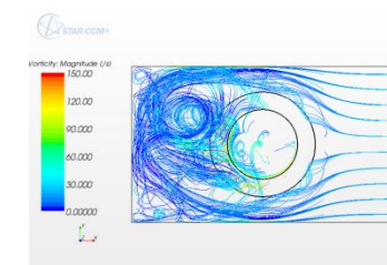
Figure 21. Streamlines from free surface k-\omega turbulence model at t=15 s
