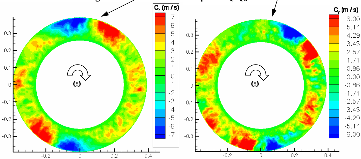
Figure 14 PIV averaging procedure results for the two modes identified at Q/Q_d = 0.45
