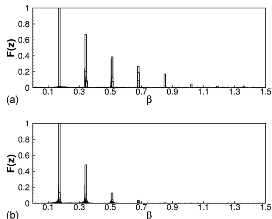
FIG. 23. Fourier transform in z at the point of maximum amplification within the separated region of the streamwise perturbation; extracted from the DNS with L_z=2\pi/\beta_{G_{\max}}=37 initialized by the two-dimensional optimal initial perturbation, at the time instants (a) t=700 and (b) t=1700 .
