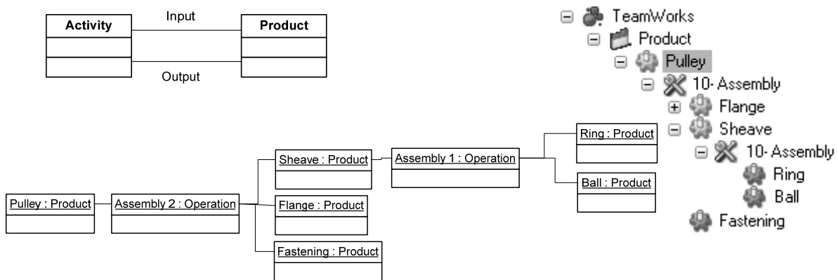
Fig. 14: UML class diagram, UML object diagram and treewiew of the manufacturing view of a product
