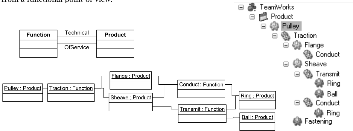
Fig. 13: UML class diagram, UML object diagram and treewiew of the functional view of a product
