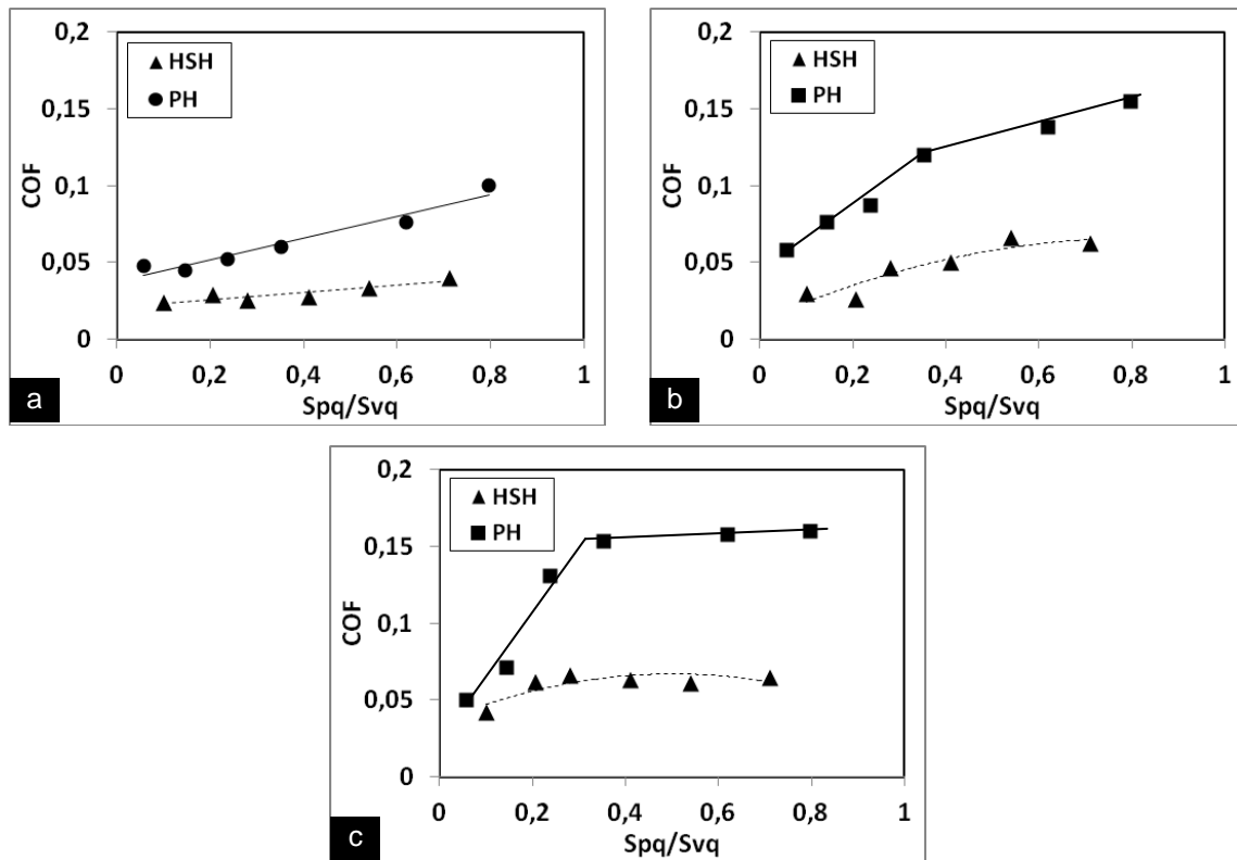
Figure 4 Friction Coefficients of PH and HSH cylinder liner surfaces function of the ratio S_{pq}/S_{vq} and for three different total surface height (a) S_z=2.5\mu m , (b) S_z=5\mu m and (c) S_z=10\mu m .
