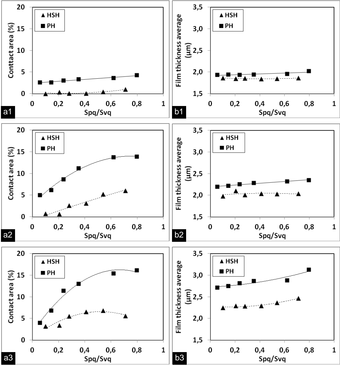
Figure 5 Contact area ratio (a) and film thickness average (b) of PH and HSH cylinder liner surfaces function of the ratio Spq/Svq and for three different total surface height (1) Sz=2.5μm, (2) Sz=5μm and (3) Sz=10μm.
