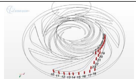
Figure 3: Probestraverses locations
