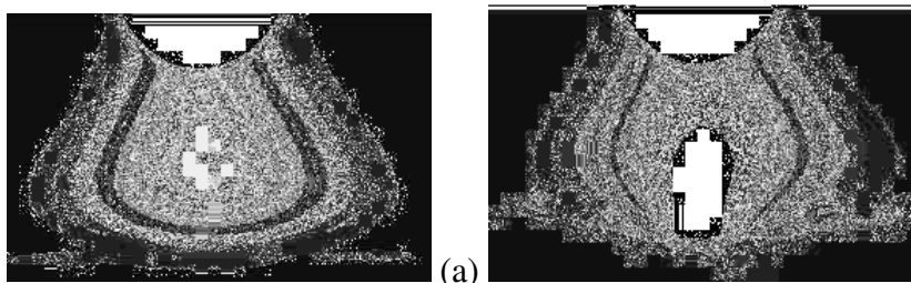
Fig.11 Stills of arc -AC TIG (a) and FBTIG (b), 150 A, 4mm gap between coatings [8]
