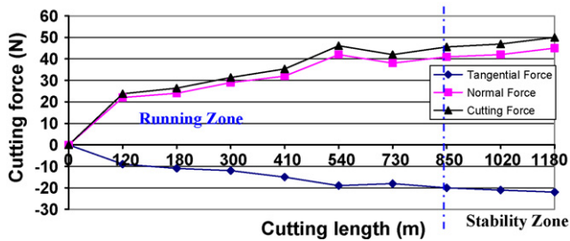
Fig. 6 – Forces variations according to the cutting length.
