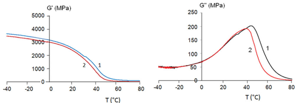
Figure 9. DMTA curves of PU samples: (1) before recovery, (2) after recovery. [Color figure can be viewed in the online issue, which is available at www.interscience.wiley.com .]
