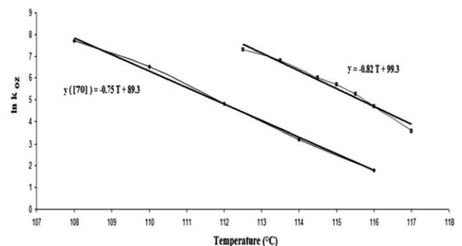
Figure 8. Ozawa constant versus temperature: comparison with Ozawa constant value from literature [70].
