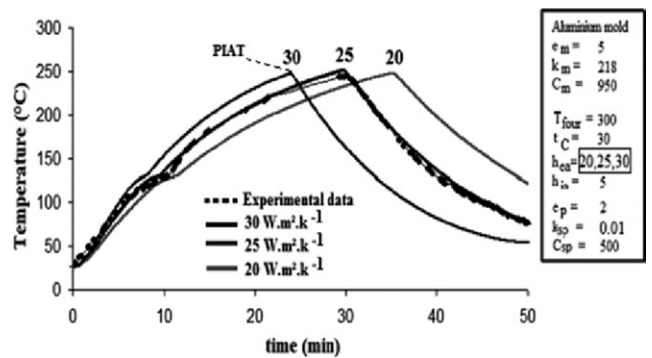
Figure 12. Numerical T-t diagrams obtained with the various coefficients of thermal transfer h_{\text{ea}} indicated ( h_{\text{ea}} = 20, 25, and 30 \text{ W m}^2 \text{ K}^{-1} , T_{\text{four}} = 300^{\circ}\text{C} ).
