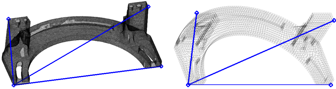
Fig. 10.(a) Measurement component mesh output by the COMET test bench. (b)Component FEM. Blue lines are orientation bases of both models for initial positioning
