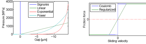
Figure 3. Sample contact (left) and friction (right) laws.
