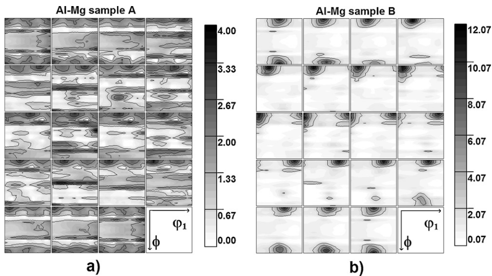
Fig. 5. Orientation distribution function (ODF) determined by X-ray diffraction for the Al-Mg samples: initial (a) and cold rolled (b). The sections through the Euler space [010] with the step of 5^\circ along the \phi_2 axis are presented.
