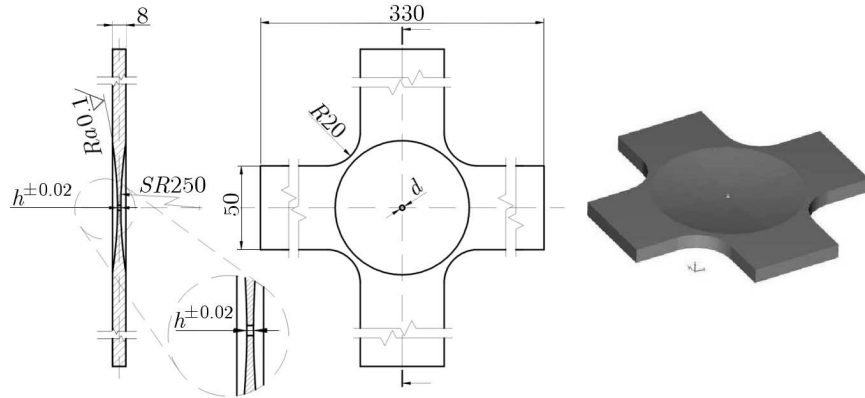
Fig. 3. Geometry of a cruciform specimen made of S355 J2G3 steel
