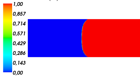
(b) iteration 5
