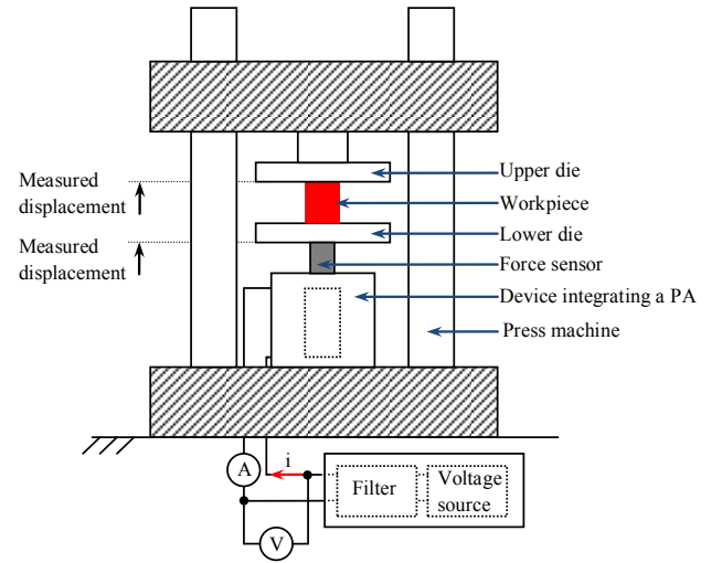
Fig. 2. Experimental setup
