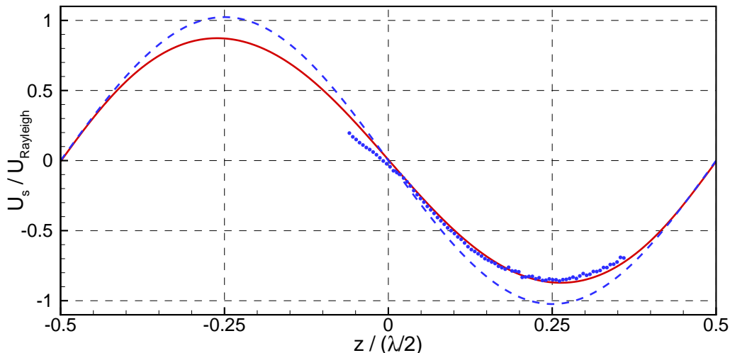
FIG. 5. (color online) Variation of the normalized axial streaming velocity component along the central axis of the guide. ( - - ) Analytical results using the conditions of the experiment ; (●) E_2 , experimental measurements at Re_{NL} = 4.8 ; (—) N_2 , numerical simulation Re_{NL} = 4.91 .
