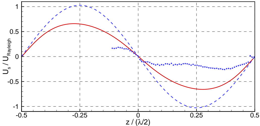
FIG. 7. (color online) Variation of the normalized axial streaming velocity component along the central axis of the guide. (---) Analytical results using the conditions of the experiment ; (•) E_4 , experimental measurements at Re_{NL} = 14.6 ; (—) N_4 , numerical simulation at Re_{NL} = 15.2 .
