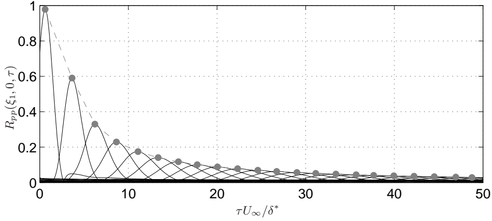
FIGURE 15. Peaks of the longitudinal space-time correlation for increasing space increments \xi_1/des=1.9 as a function of the nondimensionalised time increment \tau U_\infty/\delta^* . The grey bullets show the maximum location.
