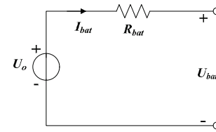
Fig. 4. Internal resistance battery model.
