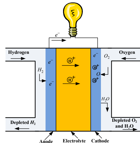
Fig.1 Schematic of an individual fuel cell
