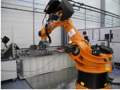
Fig. 1. Robot KUKA KR500-2MT (by courtesy of Institut de Soudure)
