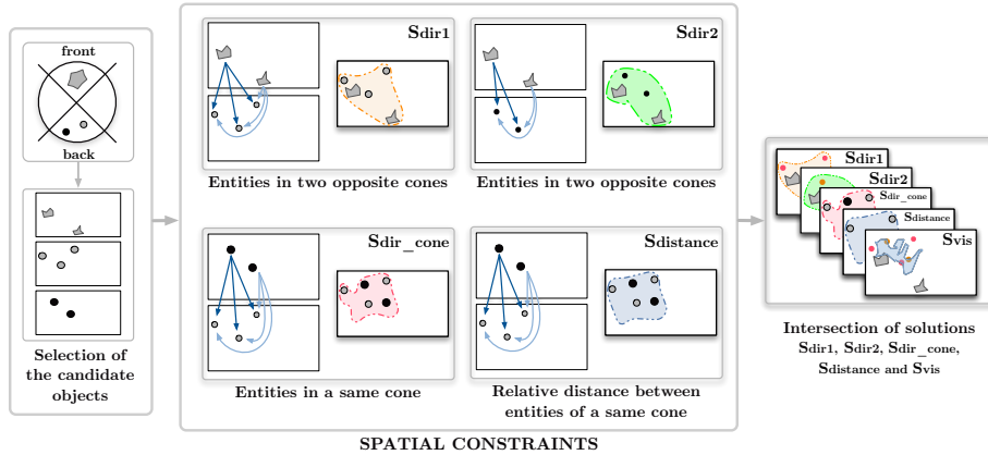
Fig. 9. Constraint-based approach
