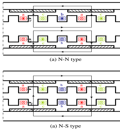
Fig.3 Flux directions for both N-N type and N-S type magnet arrangement of 2R-1S AFPM machine
