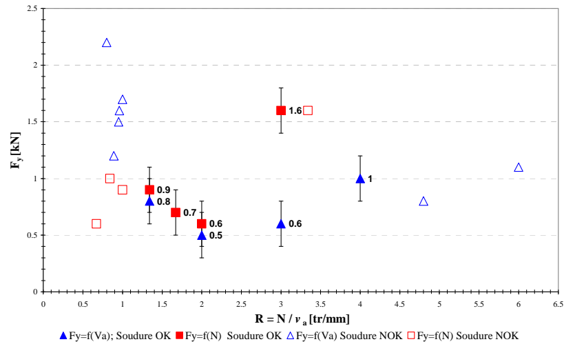
Figure 1 : Evolution de la transverse force versus rotation speed on travel speed ratio
