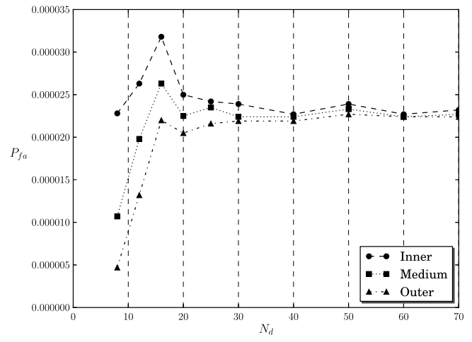
Fig. D.16. Convergence of the probability of failure of the assembly requirement for the third set of values.
