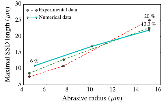
Fig. 10. Maximal SSD length versus average abrasive radius for different abrasive concentrations.
