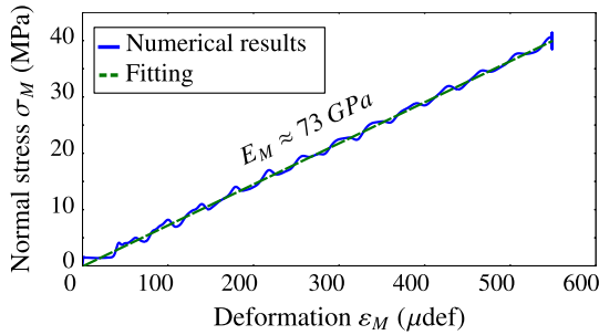
Fig. 5. Evolution of the macroscopic normal strain \varepsilon_M versus the macroscopic normal stress \sigma_M .
