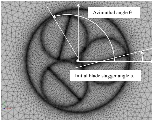
Fig. 5 Zoom of the mesh of the VAWT with straight blades
