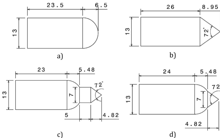
Fig. 7. Projectile shapes used during perforation tests. a) Hemispherical projectile; b) Conical projectile; c) Hemispherical + conical (projectile A); d) Hemispherical-conical (projectile B).
