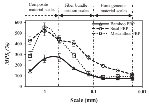
Fig. 8. Multiscale profile milling process signature for the different NFRP at f_z=0.04 mm/tooth.
