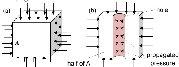
Figure 5 Pressure propagation in case of a drilling
