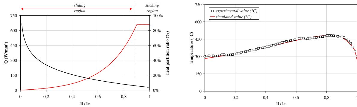
Figure 5 – Temperature distribution and heat flux free cutting steel – V_c = 110 \text{ m/min} – f = 0,4 \text{ mm/rev} – a_p = 1,5 \text{ mm}
