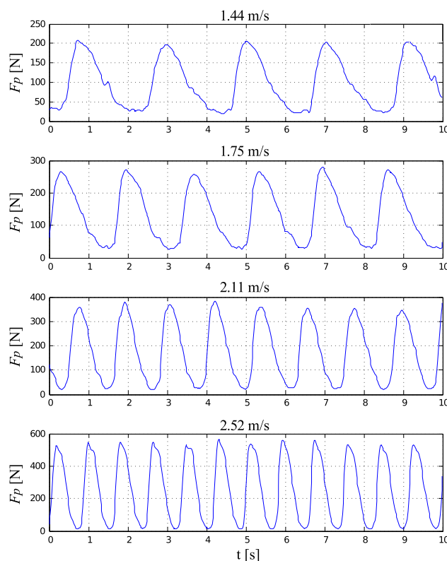
Fig. 5 Times series of the applied pedal force for different kayak speeds
