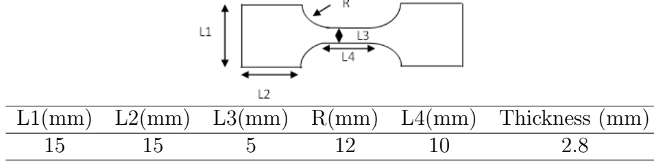
Figure 1: Specimens dimensions.
