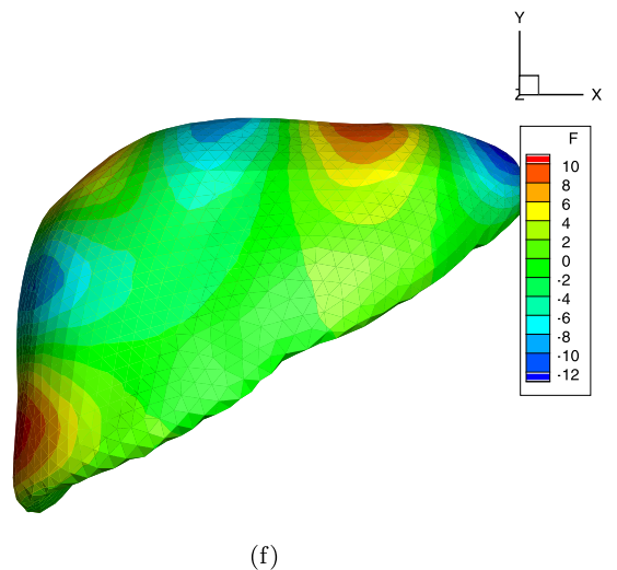
Fig. 15 Six first functions Y(y) , k = 1, \dots, 6 , for the simulation of the liver. Note that, in this case, functions Y(y) are defined on the boundary of the liver only
