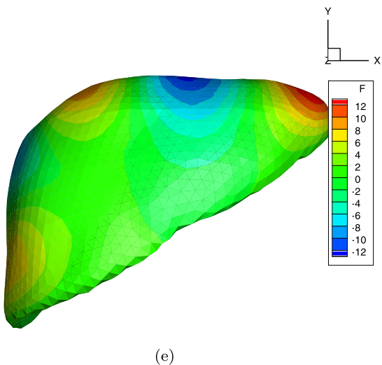
Fig. 15 Six first functions Y(y) , k = 1, \dots, 6 , for the simulation of the liver. Note that, in this case, functions Y(y) are defined on the boundary of the liver only
