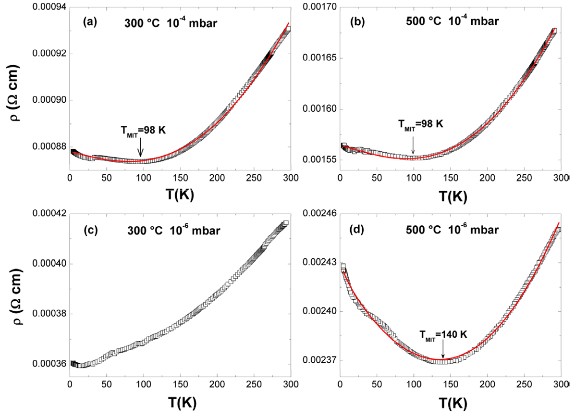
Figure 4. Temperature -dependent resistivity of Nd-doped ZnO films grown under (a) 10^{-4} at 300^\circ\text{C} , (b) 10^{-4} mbar at 500^\circ\text{C} , (c) 10^{-6} mbar at 300^\circ\text{C} , and (d) 10^{-6} mbar at 500^\circ\text{C} .
