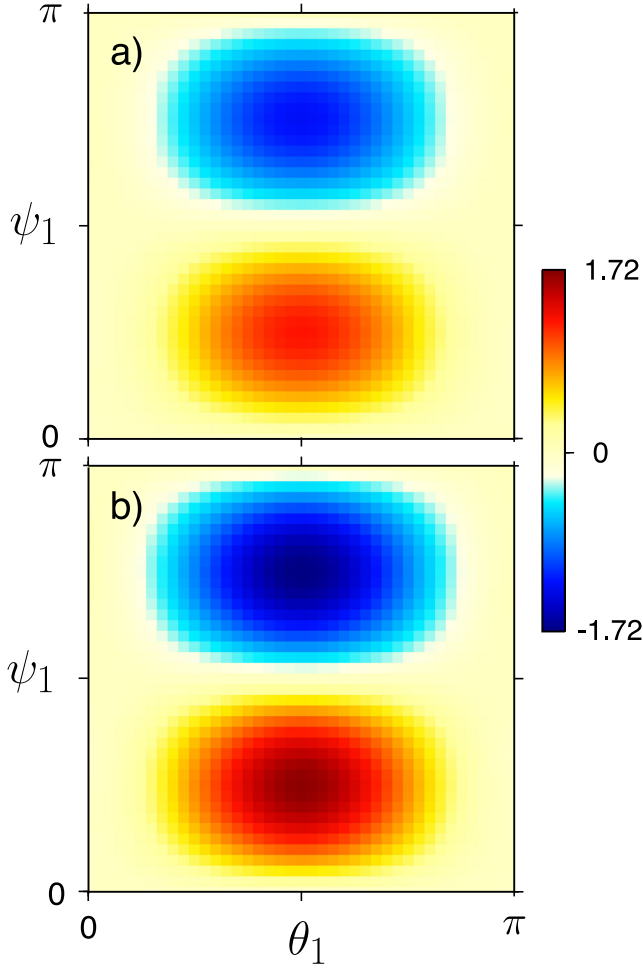
Figure 3. Instantaneous crystallographic spin \psi^{[1]}(\theta^{[1]}, \psi^{[1]}) for the slip system (010)[100], predicted by the SO model with \tau^{[1]}/\tau^{[2]} = \tau^{[2]}/\tau^{[3]} = 1 for an initially isotropic olivine aggregate deformed in uniaxial compression. (a) |\dot{\epsilon}_3|t = 0 ; (b) |\dot{\epsilon}_3|t = 0.4 . Colour scale is in units of the axial shortening rate \dot{\epsilon}_3 < 0 . The Eulerian angles \theta^{[1]} and \psi^{[1]} are defined as in Fig. 2(b).
