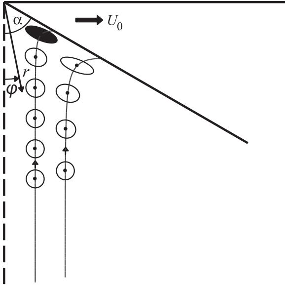
Figure 9. Geometry and boundary conditions for the corner flow model of a ridge crest (right half only). The half spreading rate is U_0 and the asthenospheric wedge has angular dimension \alpha = 60^\circ . Solid lines with arrows show typical streamlines for a power-law rheology with index n = 3 . The FSEs are plotted at different points along the two streamlines. The black ellipse relates to the point in the flow at which the texture is approximated (see Fig. 10).
