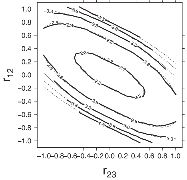
Figure 4. Spin amplitude B as a function of deformation when the strengths of the dominant slip systems are all equal, shown as a function of the axial ratios of the finite strain ellipsoid. Solid contours show the amplitude B that best fits the predictions of the SO model, and the dashed contours show the fitting function (B3).
