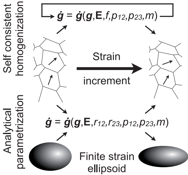
Figure 1. Schematic comparison of the analytical approach and homogenization methods for a single strain increment. Using SO to calculate the spin, \dot{\mathbf{g}} , for the n th grain and update its orientation, \mathbf{g} , requires knowledge of the strain, and thus spin, of all other crystals in the aggregate necessitating an expensive self-consistent solution. Our analytical approach replaces this information with a record of previous deformation stored as an auxiliary finite strain ellipsoid. This, combined with a handful of other parameters, A , enables rapid calculation of the spin.
