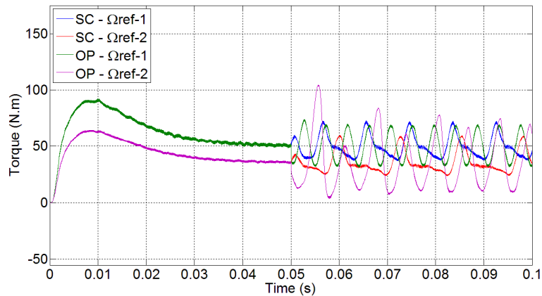
Fig. 13: Torque generated by M1 of the RIMM topology
