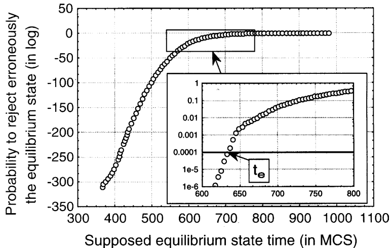
Fig. 7. Evolution of the probability to reject erroneously the equilibrium state, \Pi[S_0(t_{1, \dots, 1000, 32, 100})] , versus the supposed equilibrium time for a system size of 32^2 cells. For the values of \delta = 0.0001 , the equilibrium time is t_e = 635 .
