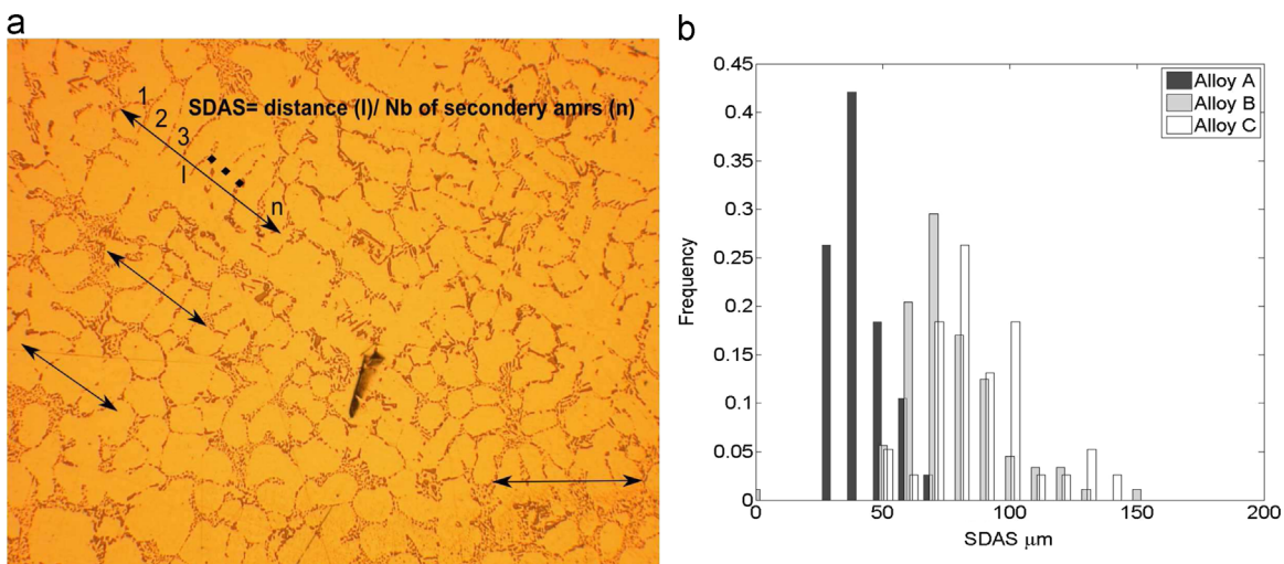
Fig. 3. SDAS measurement method (a) and the SDAS distributions of three materials under investigation (b).
