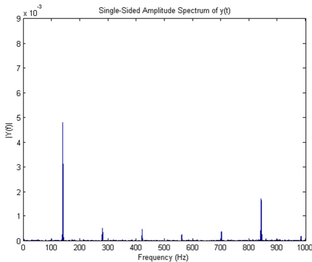
Fig. 14 Frequency spectrum of the excitation perceived by the user in his/her palm
