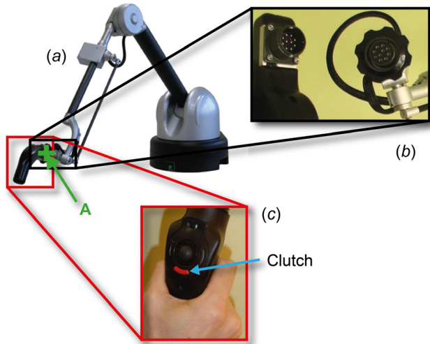
Fig. 3 Physical structure of the haptic system (a) showing the location of the end effector (c) and the connector between the arm subsystem and the standard end effector (b)
