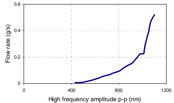
Fig. 3. Flow rate in function of HF amplitude for a corundum powder with a 15^\circ inclination of the system and Tape #1 quality of the beam surface.
