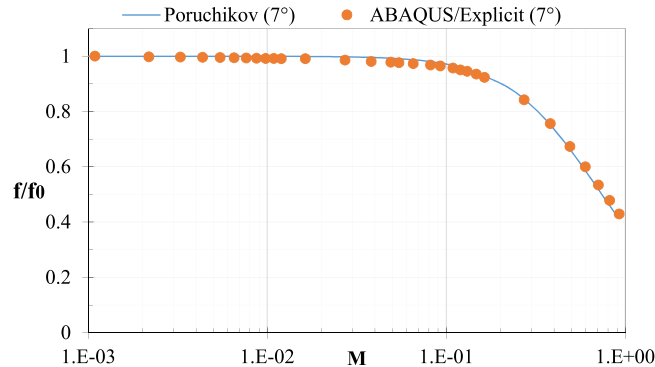
Fig. A.1. Evolution of the slamming coefficient with the Mach number in the case of the impact of a cone with a deadrise angle of 7° on pure water ( f_0 is the value of the slamming coefficient for M tending towards zero). Comparison between the analytical model of Poruchikov (1973) and ABAQUS/explicit simulations.
