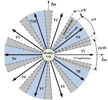
Fig.9. Fault vector average position in \alpha_f\beta_f fault reference frame according to the fault location.
