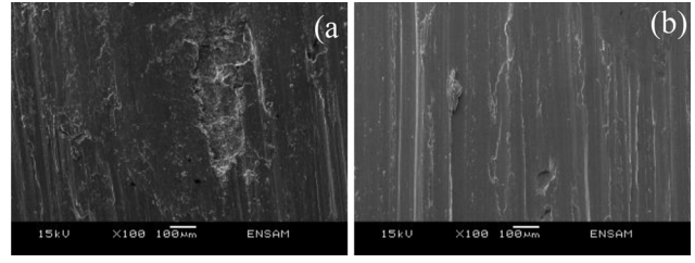
FIG. 17. SEM/SE photograph of the worn surface of the pin used with (a) Tribaloy-C1 and (b) Tribaloy-C2.
